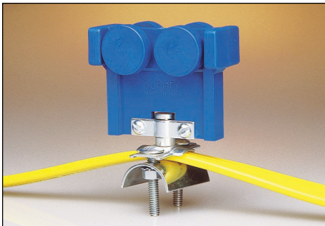
Festoon Trolley
